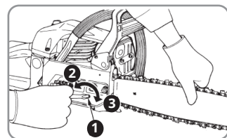
1. Tensioner screw 2. Loosen 3. Tighten
